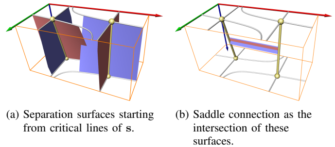
Fig. 6. Extracting saddle connections.
