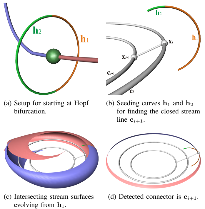
Fig. 9. Tracking closed stream lines.
