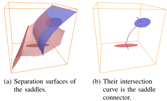
Fig. 5. Definition of saddle connectors for 3D vector fields.
