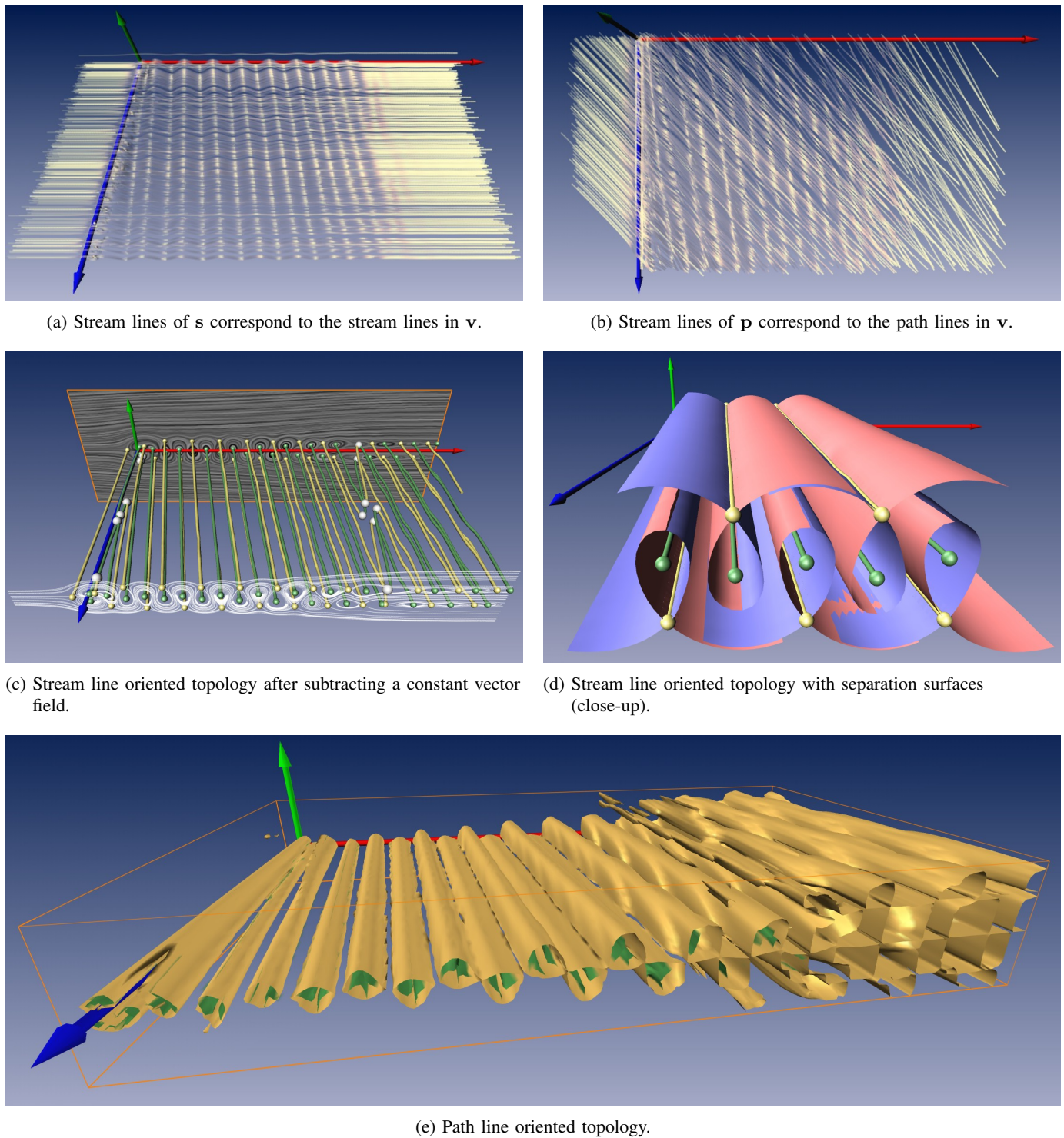
Fig. 17. 2D Flow behind a circular cylinder.
