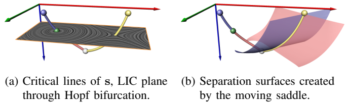
Fig. 3. Topological visualization of a simple 2D time-dependent vector field consisting of sink, source, saddle, fold and Hopf bifurcation – one of each type.
