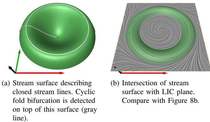
Fig. 10. Detecting a cyclic fold bifurcation.
