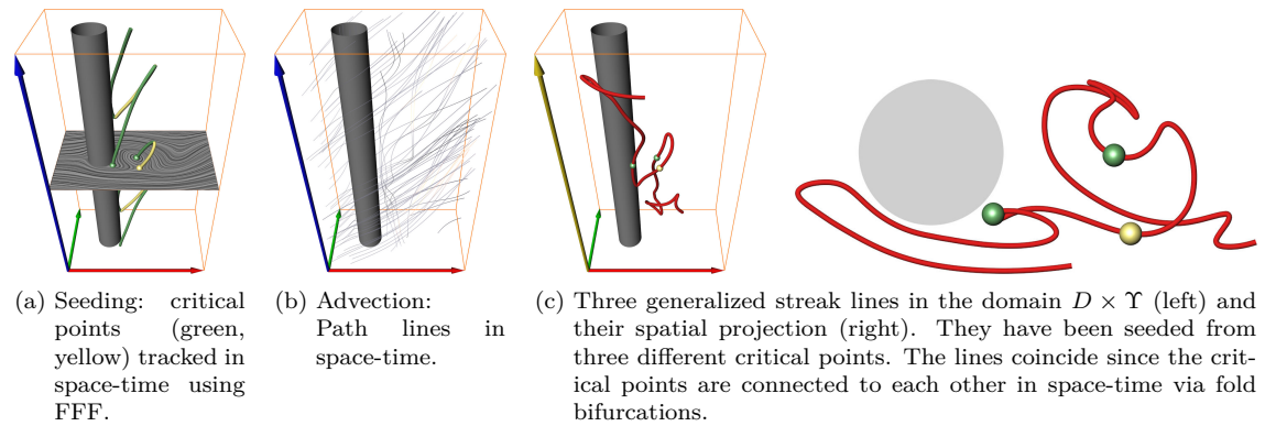
Figure 1: Generalized streak lines seeded from the locations of moving critical points in the 2D time-dependent flow behind a cylinder. The seeding field \bar{\mathbf{f}} in (a) is shown only for the tracked critical points for better visual clarity, but the whole field has been used for the computations.
